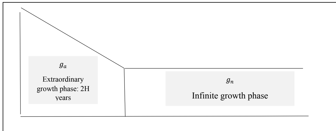
Figure 3: Expected Growth in the H Model
