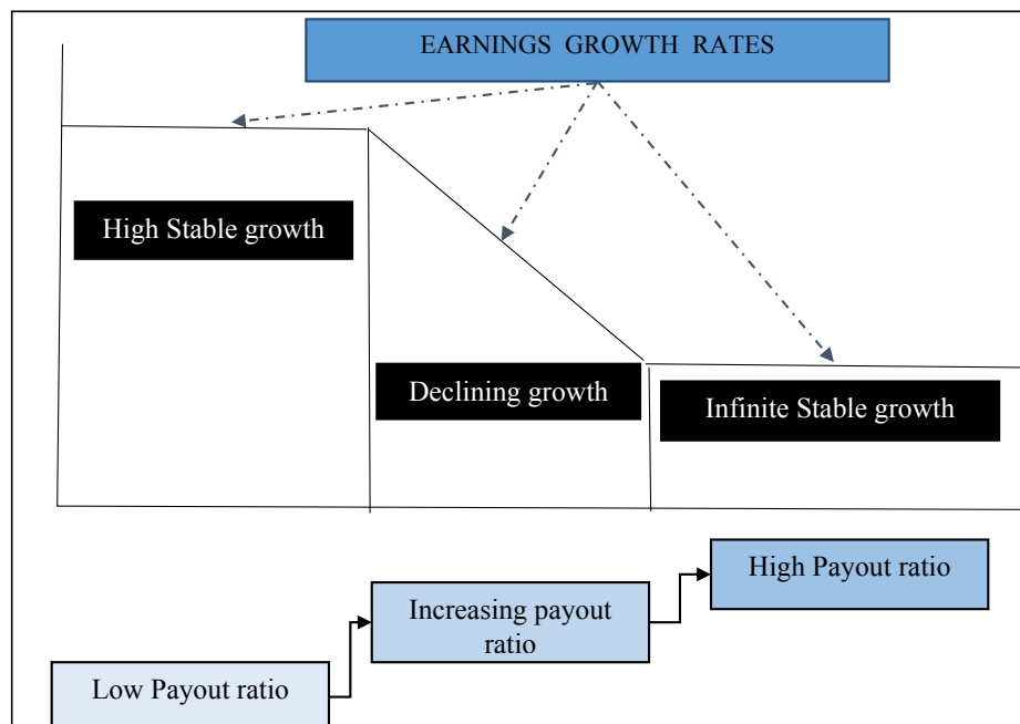
Figure 4: Expected Growth in the Three-Stage DDM
